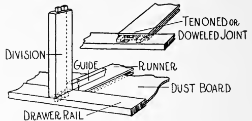
FIG. 426. DRAWER RUNNERS AND GUIDE.
